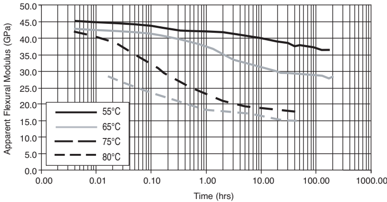
Figure 1 – Elevated Temperature Creep Data
