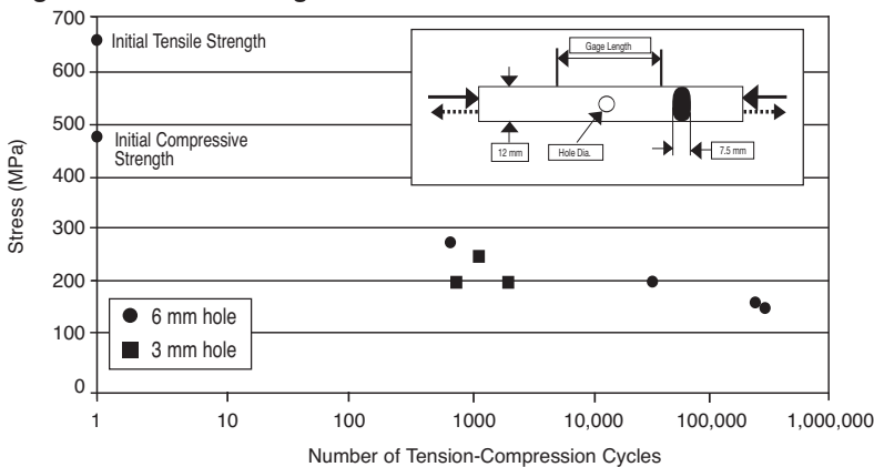
Figure 3 – Notched Fatigue
