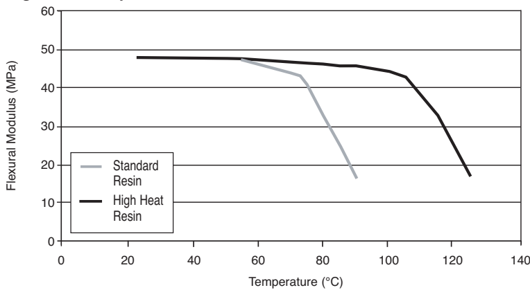
Figure 2 – Temperature Effect on Flex Modulus
